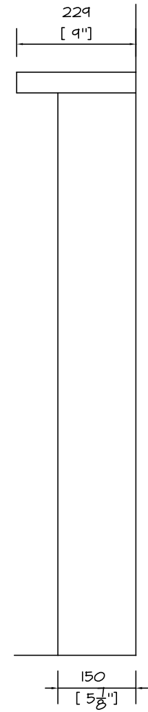
SIDE ELEVATION
